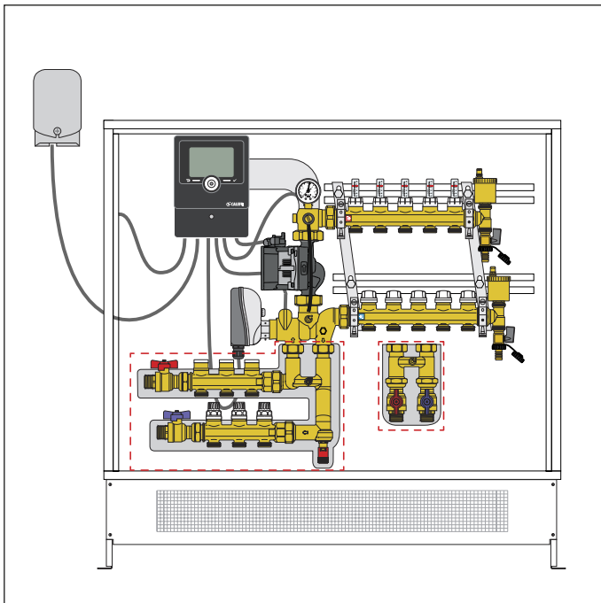
Transformation from modulating for heating to compensated temperature for heating with code 161002
