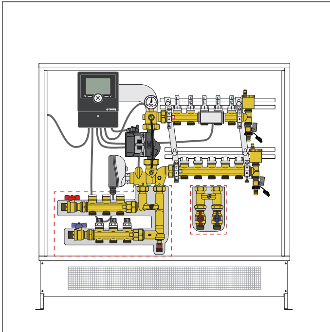
Transformation from modulating for heating to modulating for heating and cooling with code 161004
