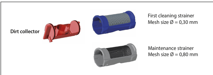
Accessory kit for circuit filling and flushing and strainer accessories for device DIRTMAGPLUS® 5453 series.
