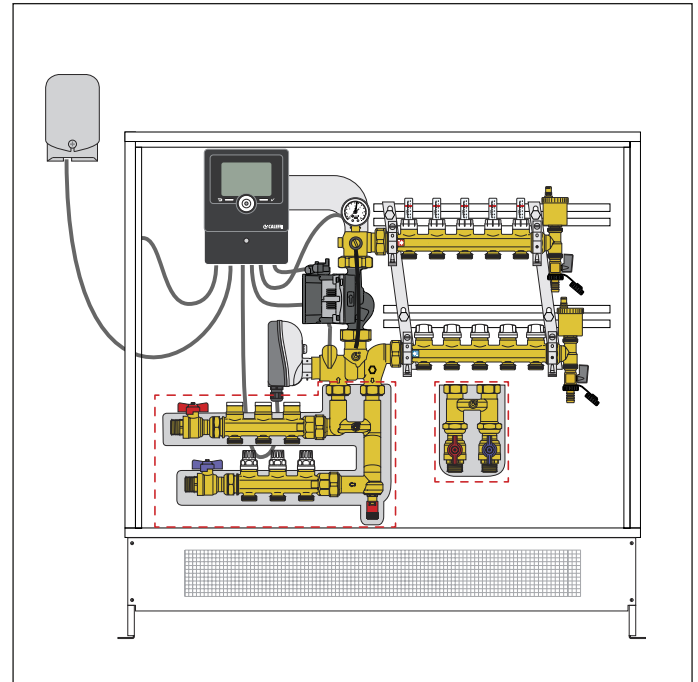
Transformation from modulating for heating to compensated temperature for heating and cooling with codes 161002 and 161004
