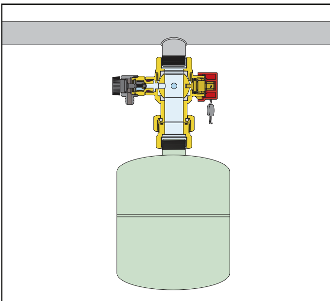
Application diagram of shut-off valve 5580 series
