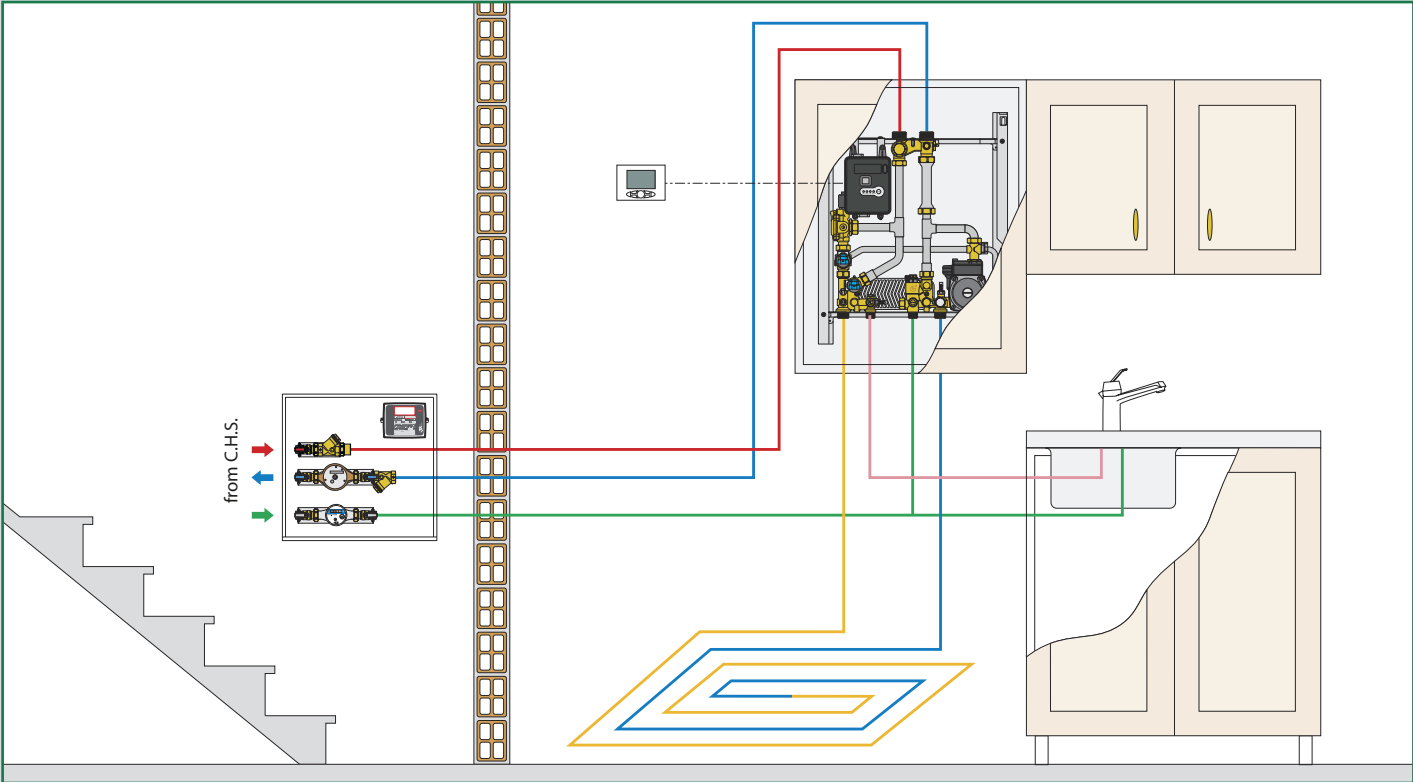
User modules Wall mounted HIU - Instantaneous DHW production Recess mounted HIU - Instantaneous DHW production
