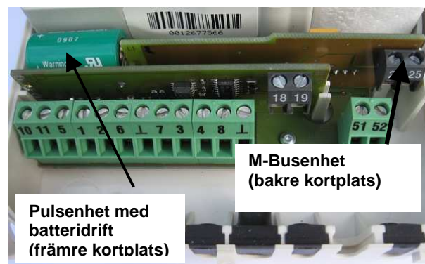
Fig. 11: Mounting modules
